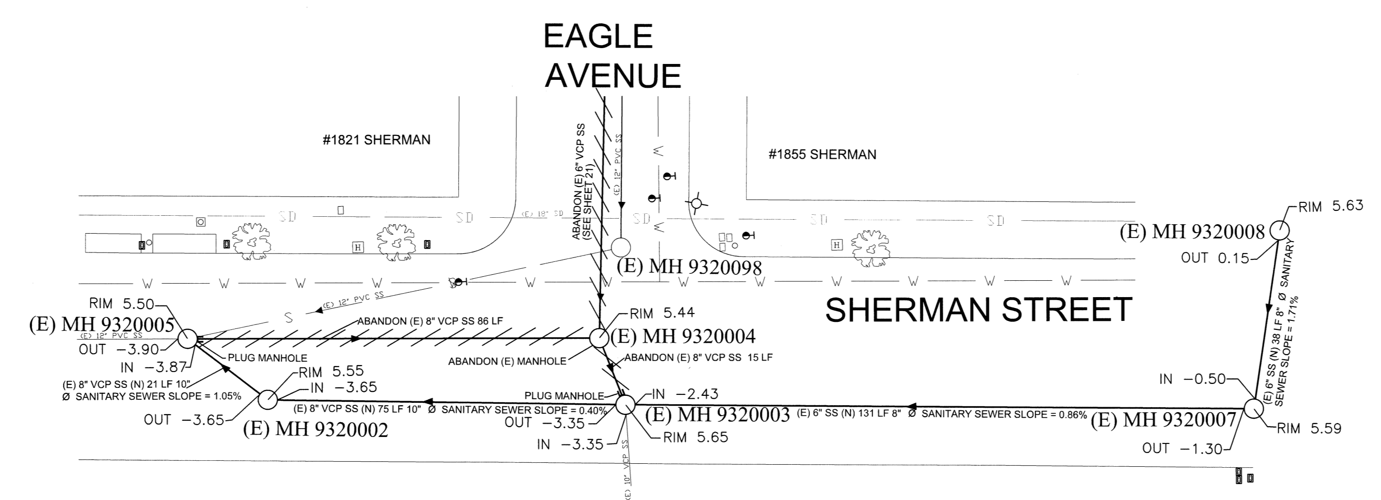
2 PLAN - SHERMAN STREET 22 SCALE: 1"=20'-0"
